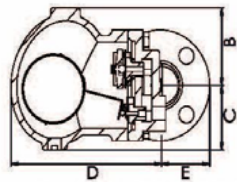
Trap No.FSX2F-FSX12F
