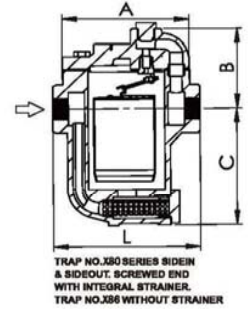
TRAP NO X80 SERIES DIMENSIONS(MM) . MOP(KG/CM 2 ).WT(KG)
