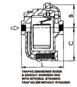
RAP NO.XS90 SERIES DIMENSIONS . MOP . & WT
